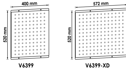
Perforated tool panel plate for tool trolleys
